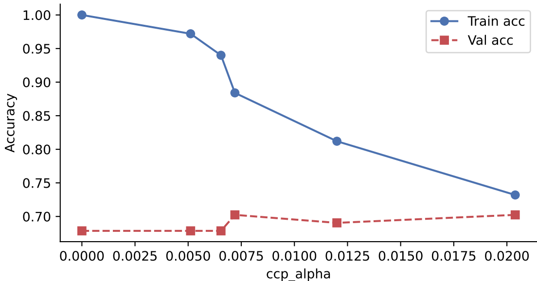
Cost-Complexity Pruning: Overfitting Mitigation
